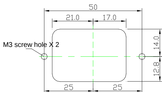
Panel Cut-out Size
