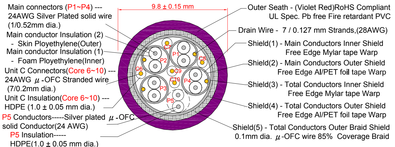
HDMI-xv1.3 Cable Construction
