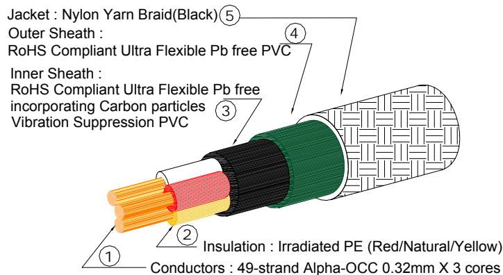
Power Ref.III Cable Construction
