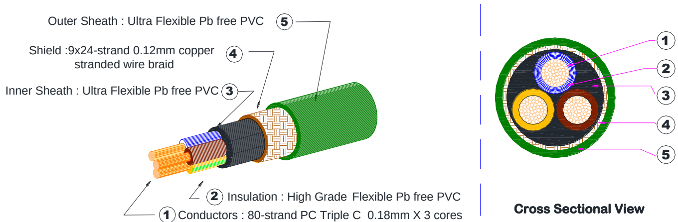
FP-TCS21 Cable Construction
