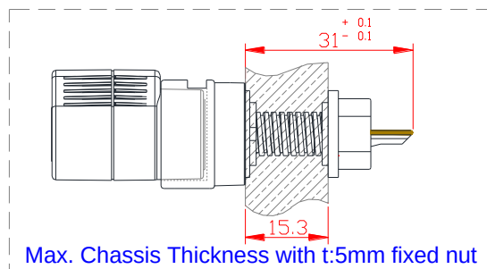
FT-867 Dimensions in mm for reference
