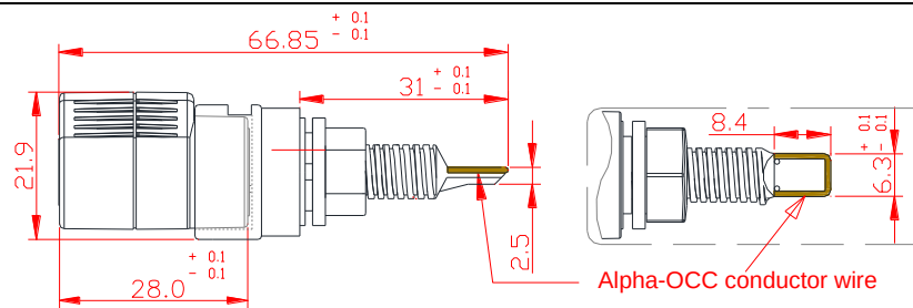
FT-867 Dimensions in mm for reference
